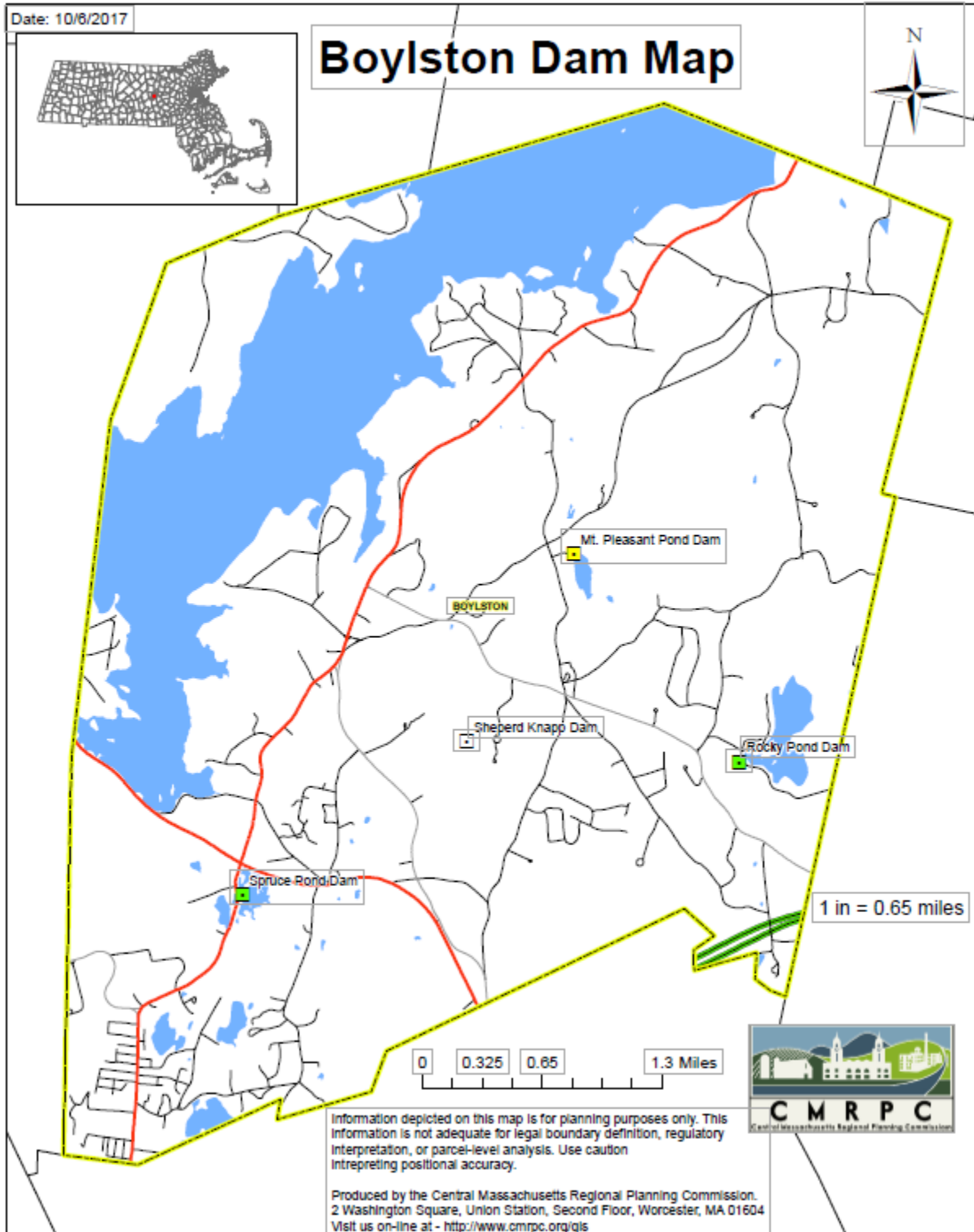
Figure 6 – Boylston Dam Locations
