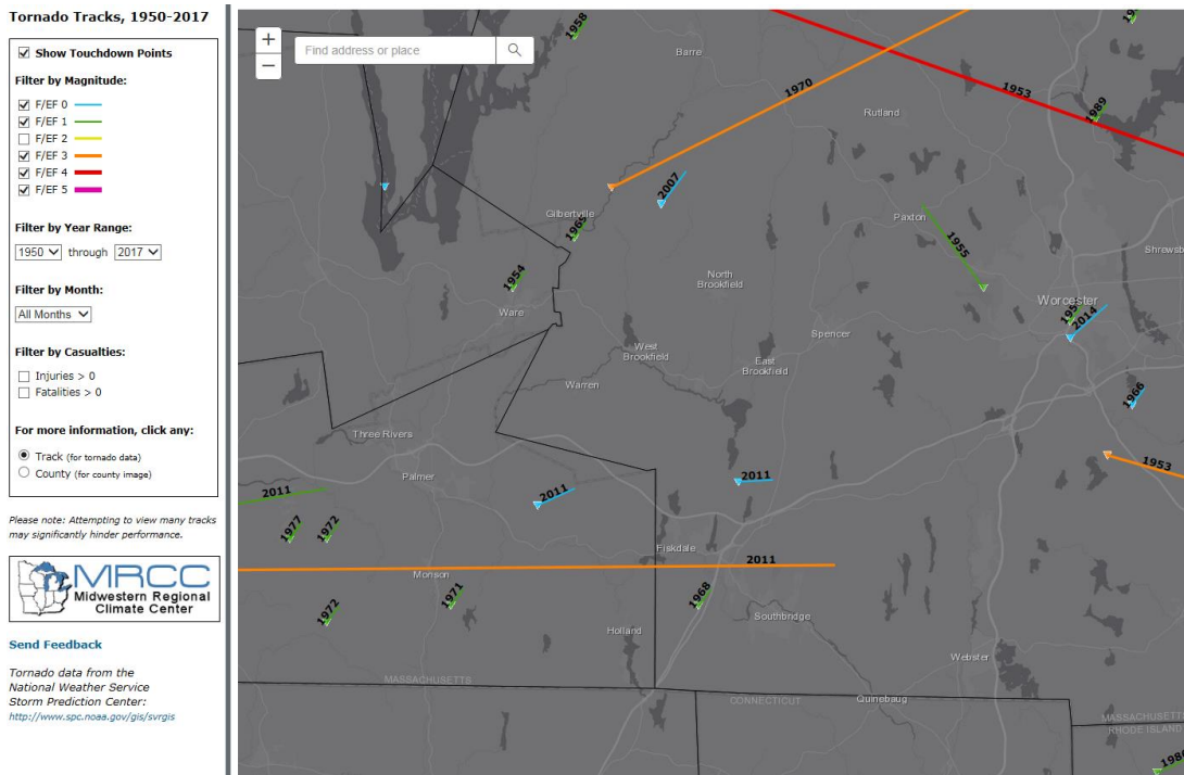
Figure - Tornado Tracks, 1950-2016 in the Leicester area. http://mrcc.isws.illinois.edu/gismaps/cntyorn.htm
