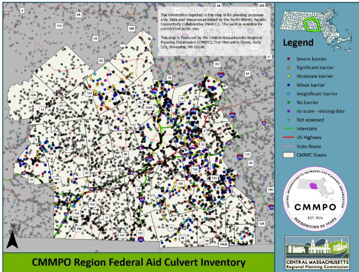
Figure 46 NAACC Culvert Aquatic Passability Scoring Results
